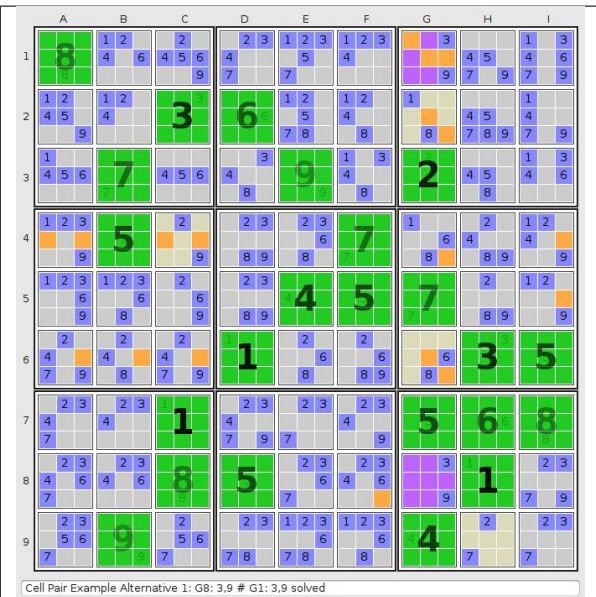
Fig. 2: Cell Pair Example Alternative 1: G8: 3,9 # G1: 3,9 solved
