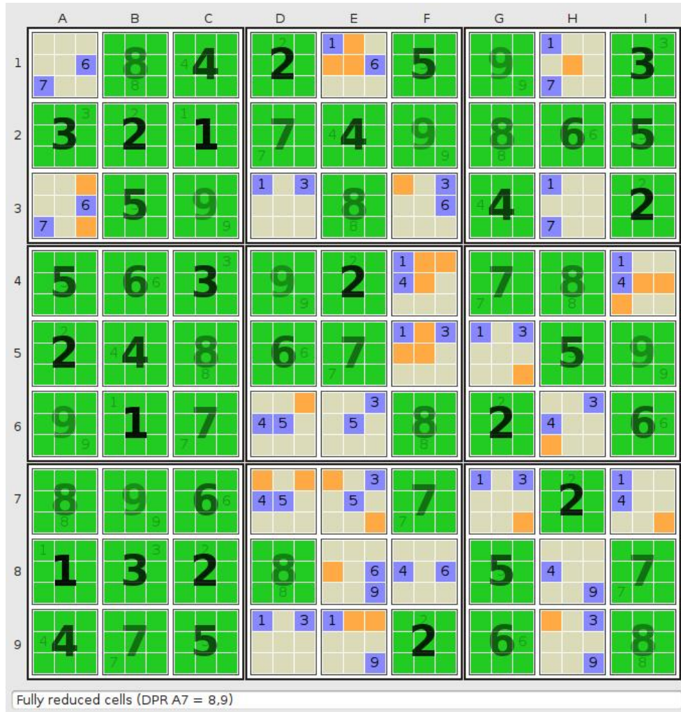
Fig. 5: Fully reduced cells (DPR A7 = 8,9)
