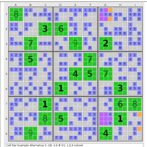
Fig. 4: Cell Pair Example Alternative 2: G8: 3,9 # G1: 1,5,6 solved
