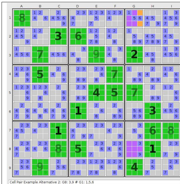
Fig. 3: Cell Pair Example Alternative 2: G8: 3,9 # G1: 1,5,6
