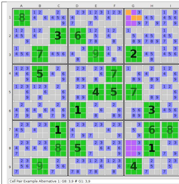
Fig. 1: Cell Pair Example Alternative 1: G8: 3,9 # G1: 3,9
